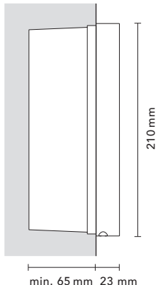
Flush mount (FM-Box)
