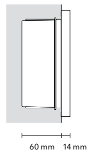
Flush mount (FM-Box)
