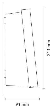
Wandmontage (WM-Box)
